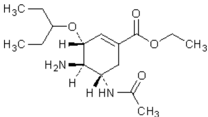
F. ethyl (3R,4R,5S)-5-(acetylamino)-4-amino-3-(1-ethylpropoxy)cyclohex-1-ene-1-carboxylate.
