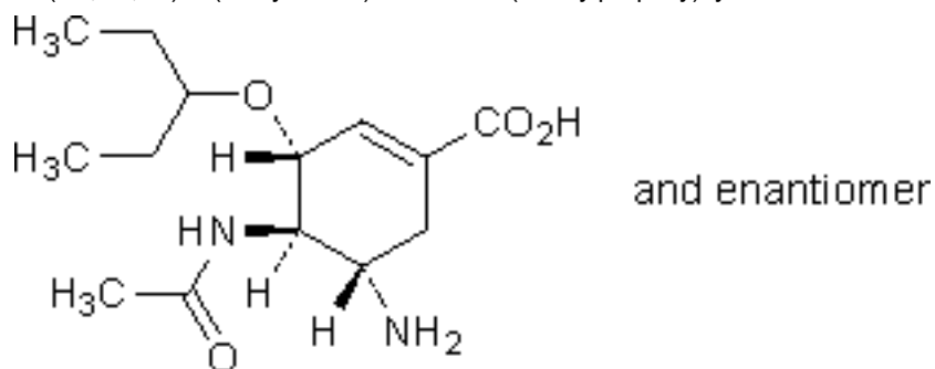
B. (3 RS ,4 RS ,5 SR )-4-(acetylamino)-5-amino-3-(1-ethylpropoxy)cyclohex-1-ene-1-carboxylic acid,
