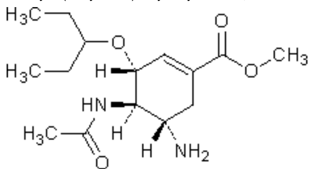
D. methyl (3 R ,4 R ,5 S )-4-(acetylamino)-5-amino-3-(1-ethylpropoxy)cyclohex-1-ene-1-carboxylate,
