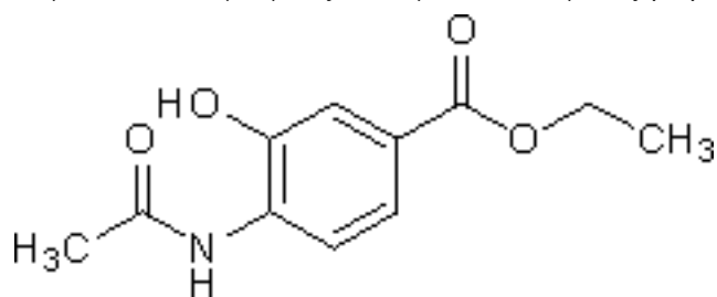
C. ethyl 4-(acetylamino)-3-hydroxybenzoate,
