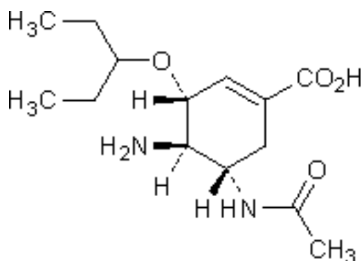
A. (3 R ,4 R ,5 S )-5-(acetylamino)-4-amino-3-(1-ethylpropoxy)cyclohex-1-ene-1-carboxylic acid
