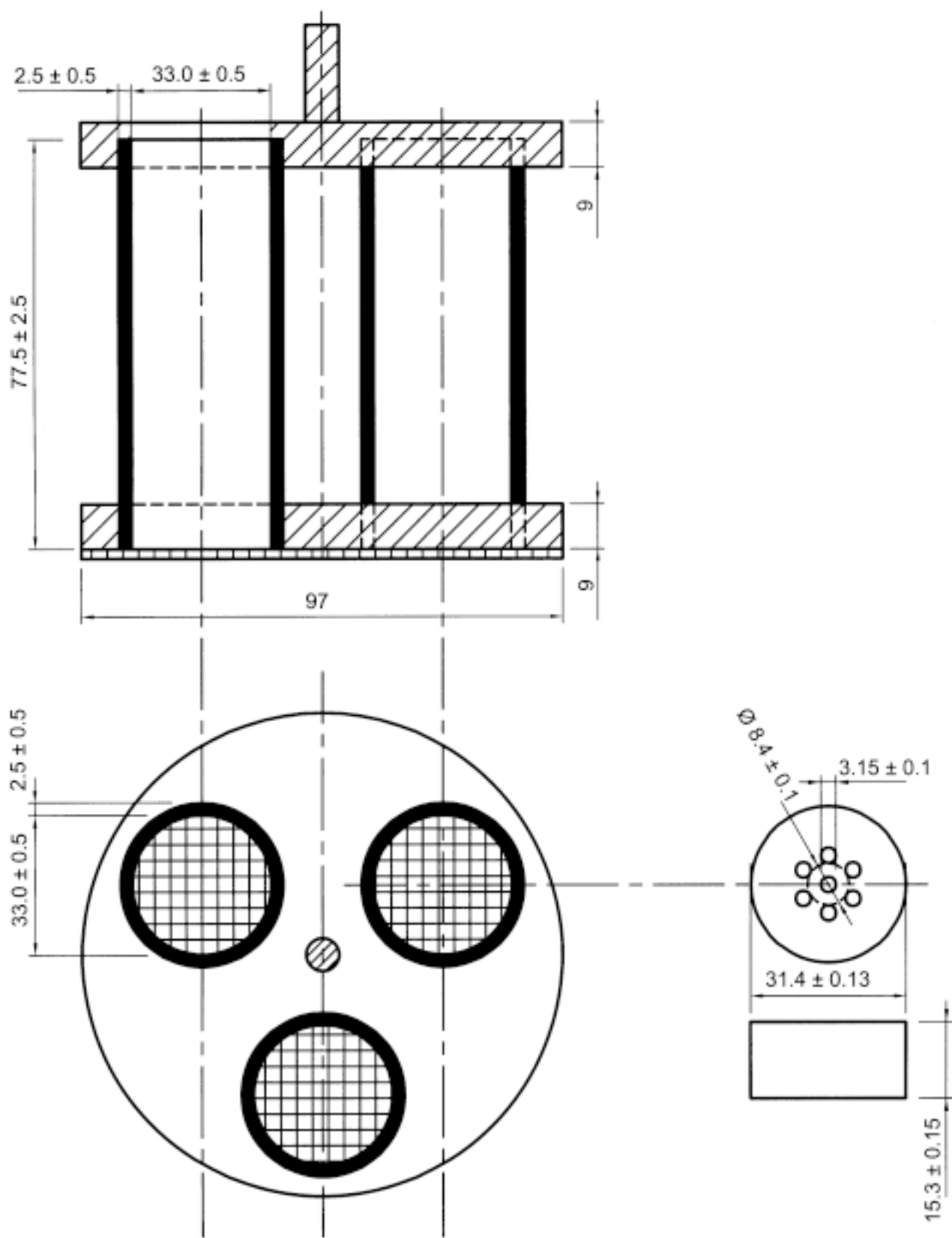
Figure 2.9.1.-2. - Disintegration apparatus B Dimensions in millimetres
